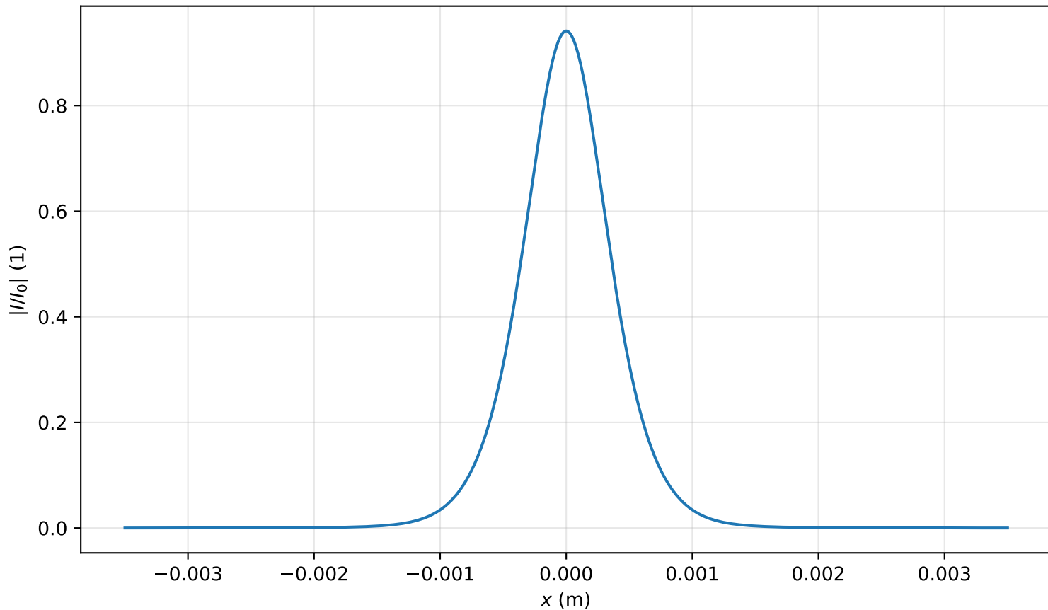
Intensity profile I(x, y = 0, z = 3.662m)/I_0 , P_{in}=0.8P_{cr} , artificial time
